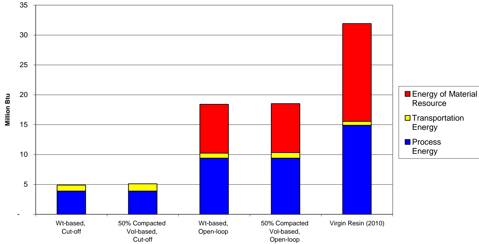
Figure 3-1b. Energy Results by Energy Category for Production of Recycled PET Resin Flake (million Btu per 1,000 pounds of resin)
